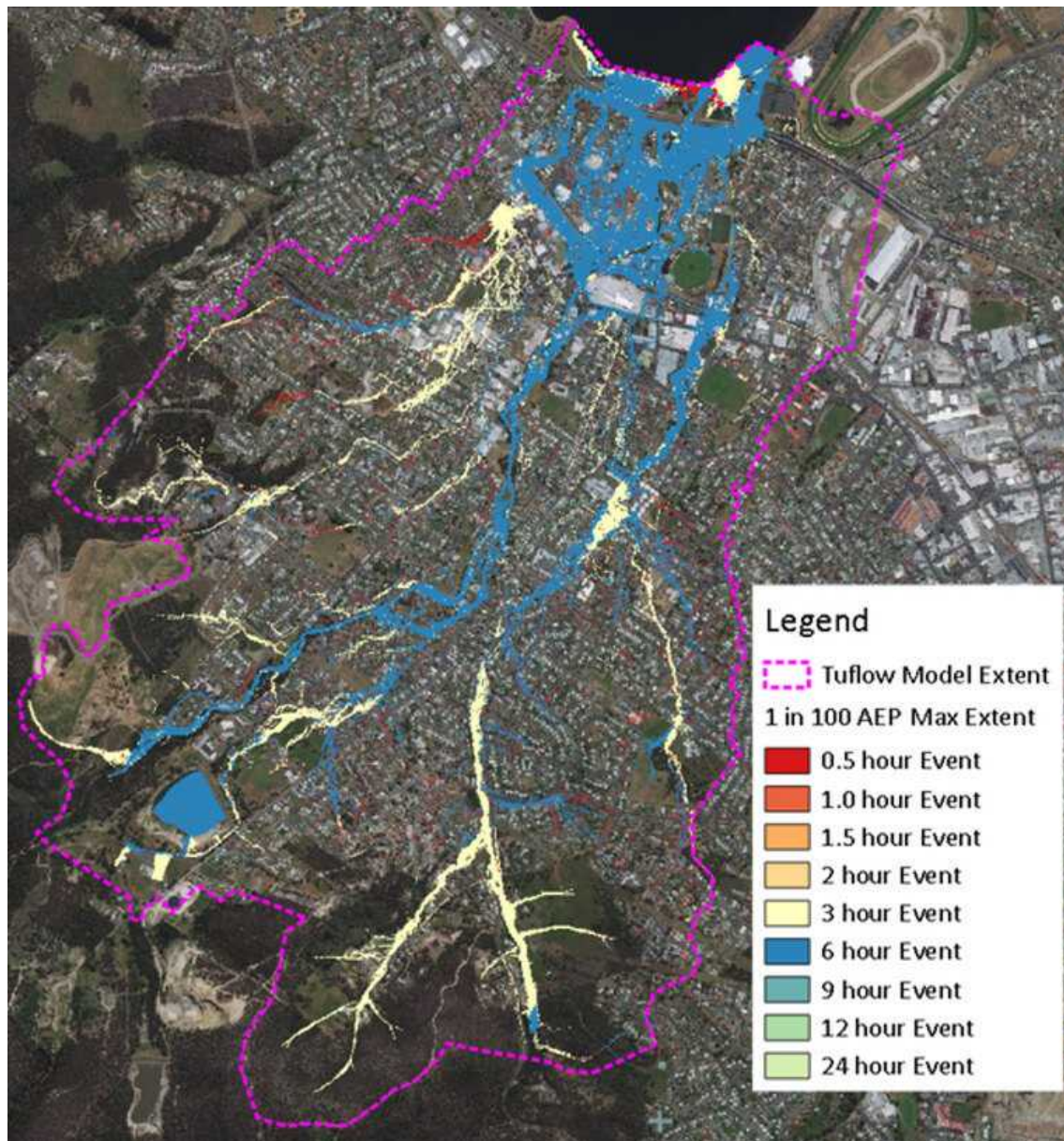
Figure 6-2 – Critical Event Map for Existing Scenario 1 in 100 AEP Inundation Event
