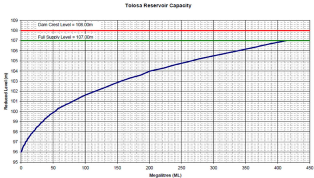
Figure C-7-6: Tolosa Reservoir Elevation Storage Relationship (SMEC 2017)
