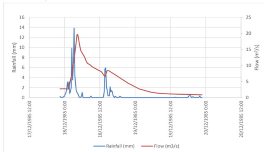
Figure 4-3 – Observed Rainfall-Runoff Event
