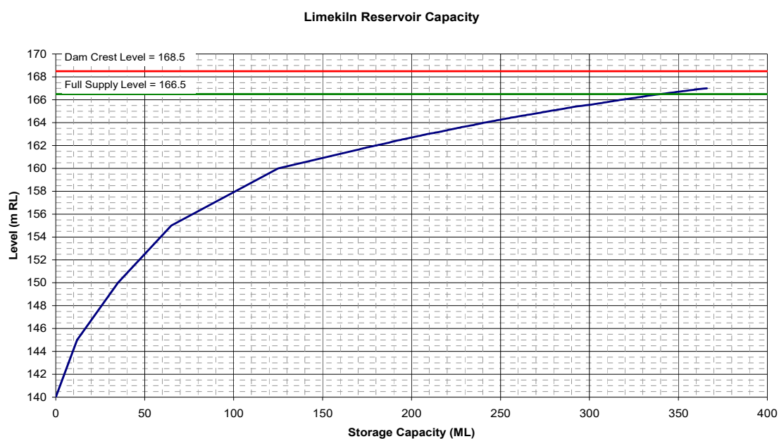
Figure C-7-4: Limekiln Gully Elevation Storage Relationship (SMEC 2017)
