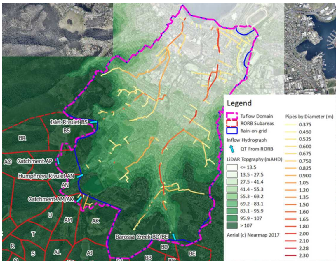
Figure 4-5 –Tuflow model Layout
