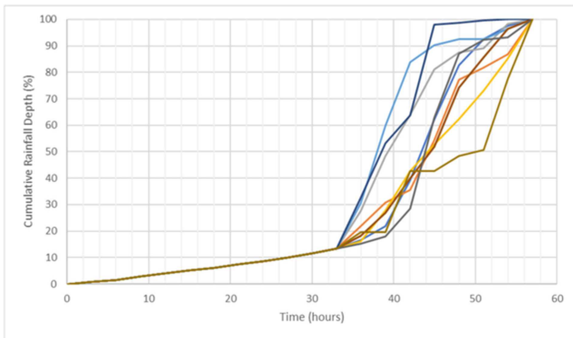
Figure 3-5 – 24 hour duration PMP ensemble of temporal patterns
