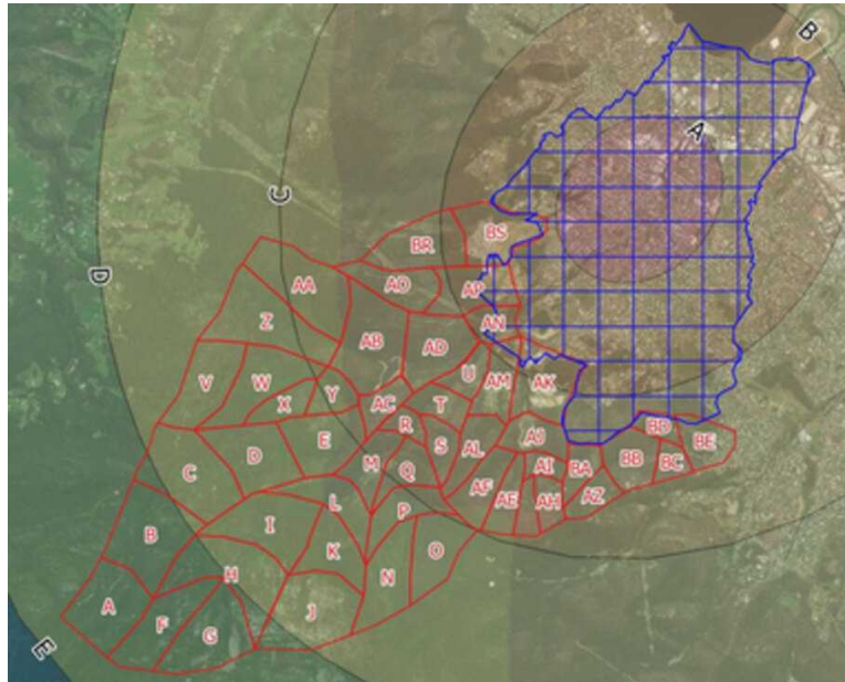
Figure 3-9 – GSDM spatial pattern centred on Glenorchy CBD.
