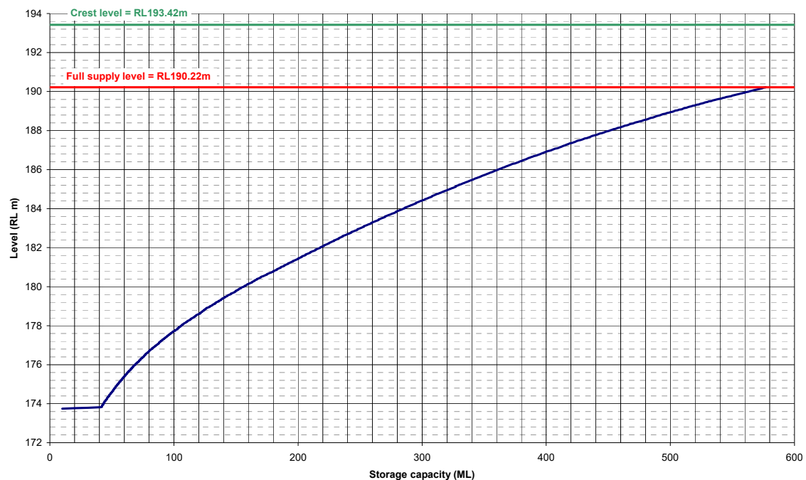
Figure C-7-1: Knights Creek Elevation Storage Relationship (SMEC 2017)
