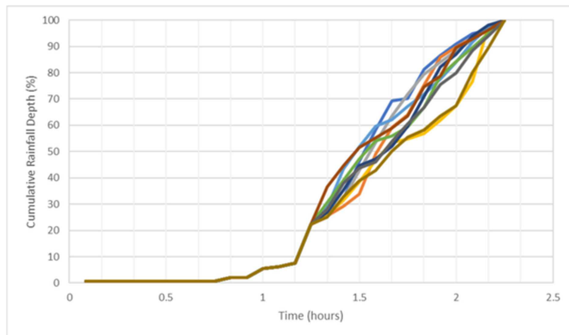
Figure 3-3 – 1 hour duration 1 in 20 AEP ensemble of temporal patterns
