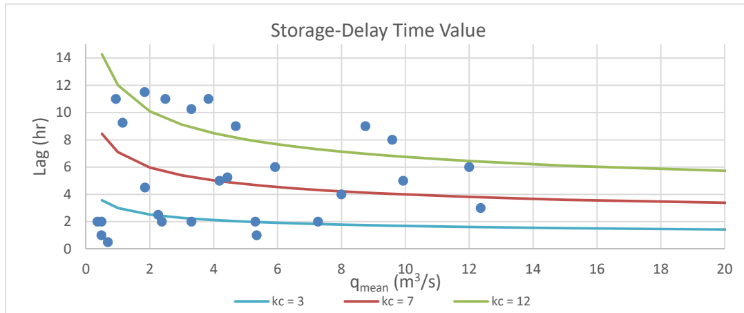
Figure 4-4 – Hobart Rivulet Observed Storm Delay
