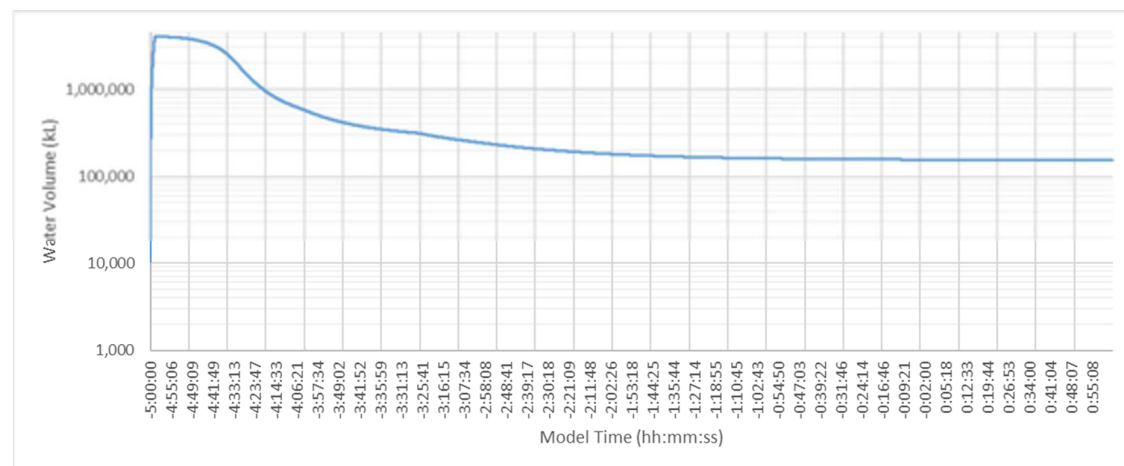
Figure 4-8 – Analysis of LiDAR depression storage volume
