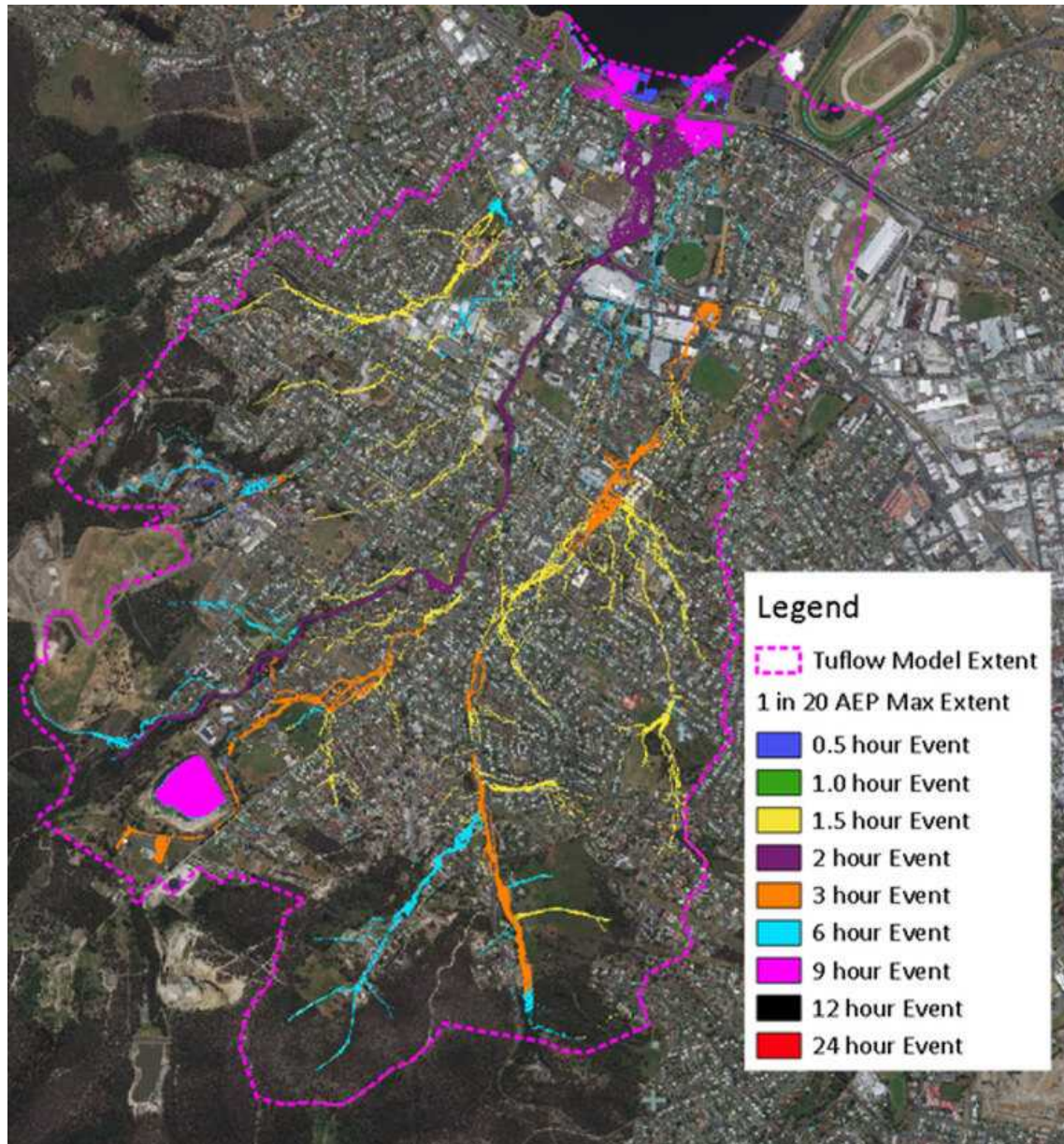
Figure 6-1 – Critical Event Map for Existing Scenario 1 in 20 AEP Inundation Event
